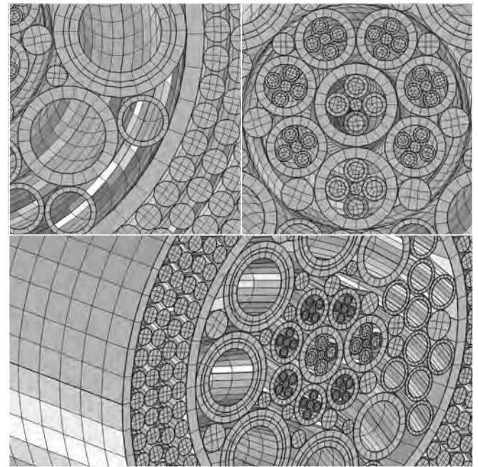
Finite Element Analysis (FEA) mesh.
