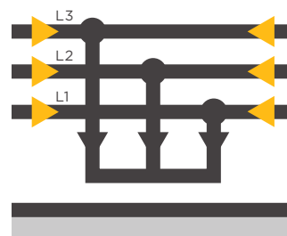
Fig 4. Three-phase short circuit
