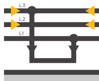
Fig 2. Phase-phase short circuit clear of earth
