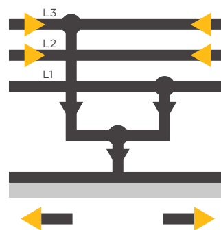
Fig 3. Phase-phase-to-earth short circuit
